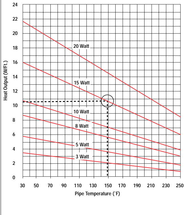
Graph 2 — SRM/E Cable Output Thermal Output Ratings On Insulated Metal Pipe
